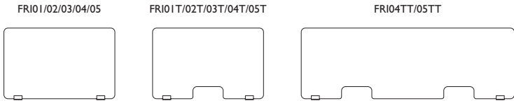
FR101 L 80 H 71 FR102 L 110 H 71 FR103 L 130 H 71 FR104 L 160 H 71 FR105 L 190 H 71 con 1 tacca passacarte / with 1 document pass-through slot FR101T L 80 H 71 FR102T L 110 H 71 FR103T L 130 H 71 FR104T L 160 H 71 FR105T L 190 H 71 con 2 tacche passacarte / with 2 document pass-through slots FR104TT L 160 H 71 FR105TT L 190 H 71
